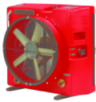
DN 800 High Expansion Foam Generator
